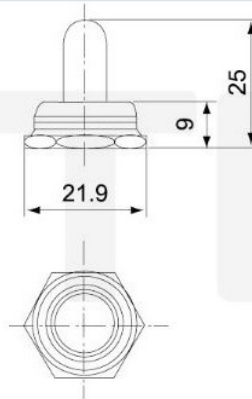
COW 防水套 Rainproof cap (Tow)
