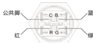
J22/25灯珠触点说明 Lamp bead contact description
