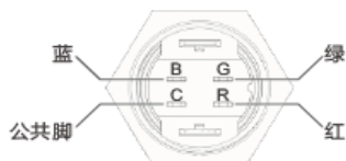
J16/19灯珠触点说明 Lamp bead contact description
