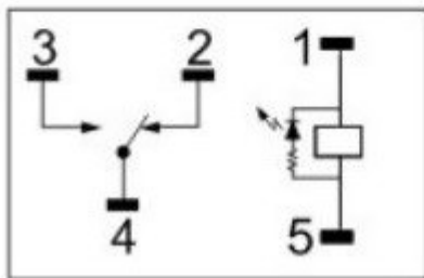
Wiring Diagram
