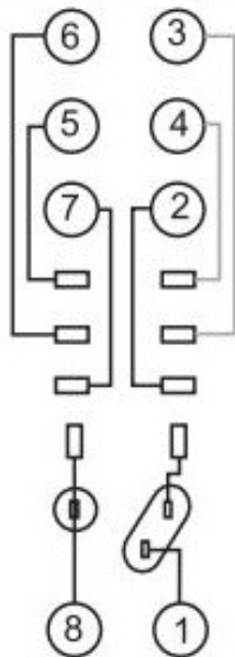
Wiring Diagram
