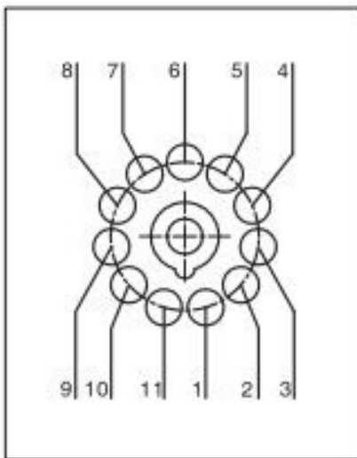
Wiring Diagram
