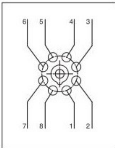
Wiring Diagram
