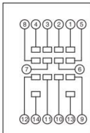
Wiring Diagram
