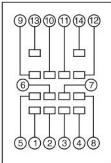
Wiring Diagram
