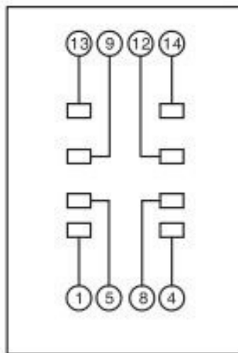
Wiring Diagram
