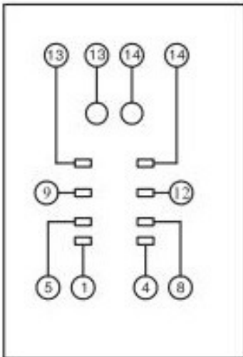
Wiring Diagram
