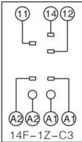
Wiring Diagram
