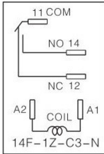
Wiring Diagram
