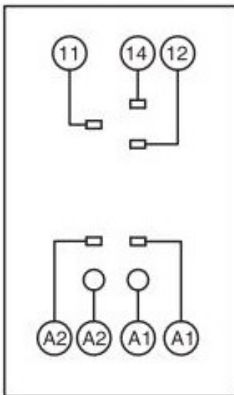
Wiring Diagram
